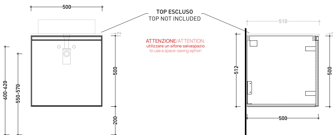
vista frontale / frontal view
