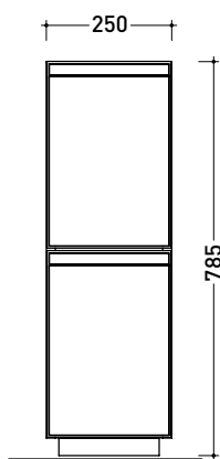
vista frontale / frontal view
