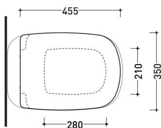
art. MN117 vista zenitale / zenital view
