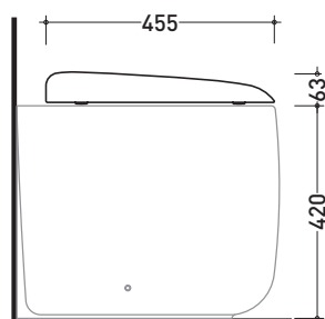
art. MN117 vista laterale / lateral view
