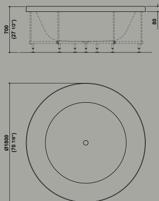
Geo 180 incasso _ built-in
