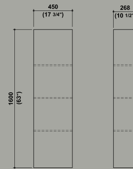
Morphing/unit colonna sospesa con anta a specchio wall unit with mirrored door
