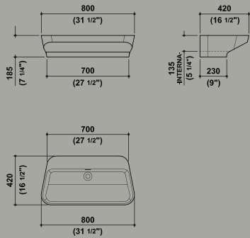
Lab 02 sospeso/appoggio _ wall mounted/deck mounted
