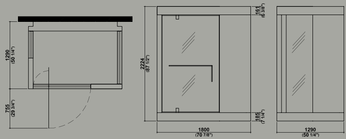
Kosmic Z2 angolo sx/dx e parete _ left/right hand and back panel to wall
