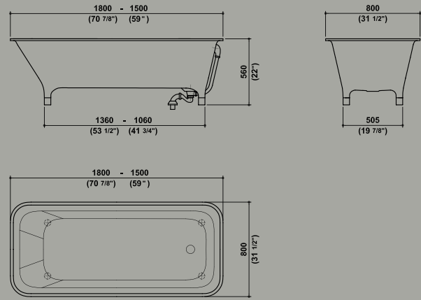
Morphing L. 1800 vasca free standing_free standing bath tub Morphing L. 1500 vasca free standing_free standing bath tub
