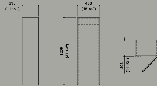
Faraway mobile in legno con anta _ folding wooden furniture
