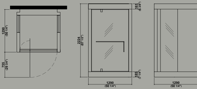
Kosmic Z1 angolo sx/dx e parete _ left/right hand and back panel to wall
