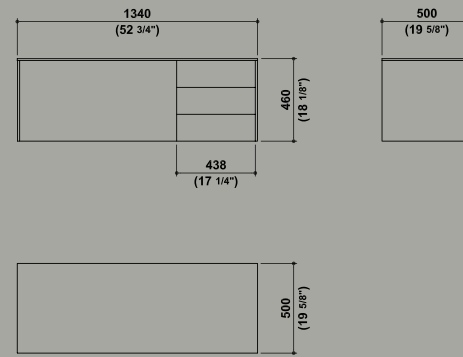
Morphing/unit mobile sospeso con cassettone e cassetteria wall-mounted base unit with pull-out drawer and 3 drawers
