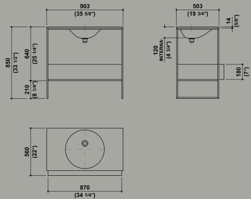
Morphing/steel mobile con lavabo integrato e cassetto console with integrated washbasin and drawer
