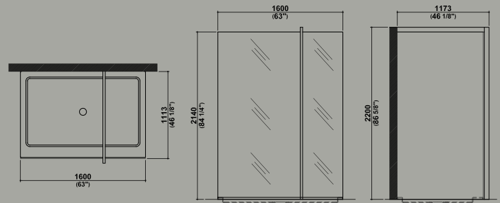
Floor 2 sistema doccia _ shower system
