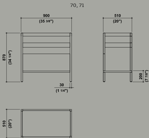
Faraway console in legno _ wooden console
