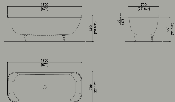
Geo 170x70 incasso _ built-in Geo 180x80 incasso _ built-in
